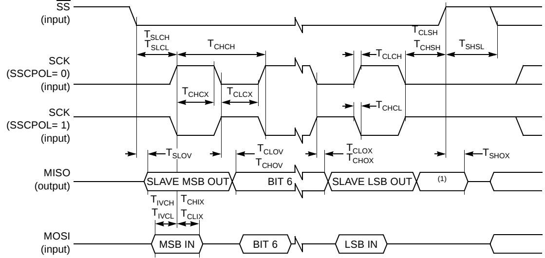
Figure 158. SPI Slave Waveforms (SSCPHA= 0)
