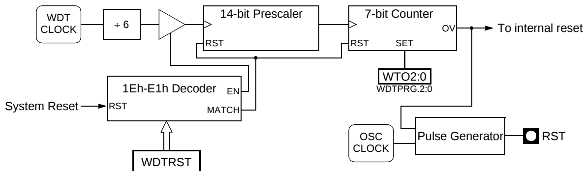
Figure 36. WDT Block Diagram
