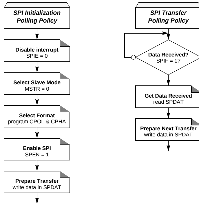
Figure 112. Slave SPI Polling Flows
