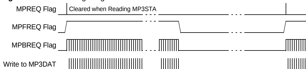
Figure 41. Data Timing Diagram
