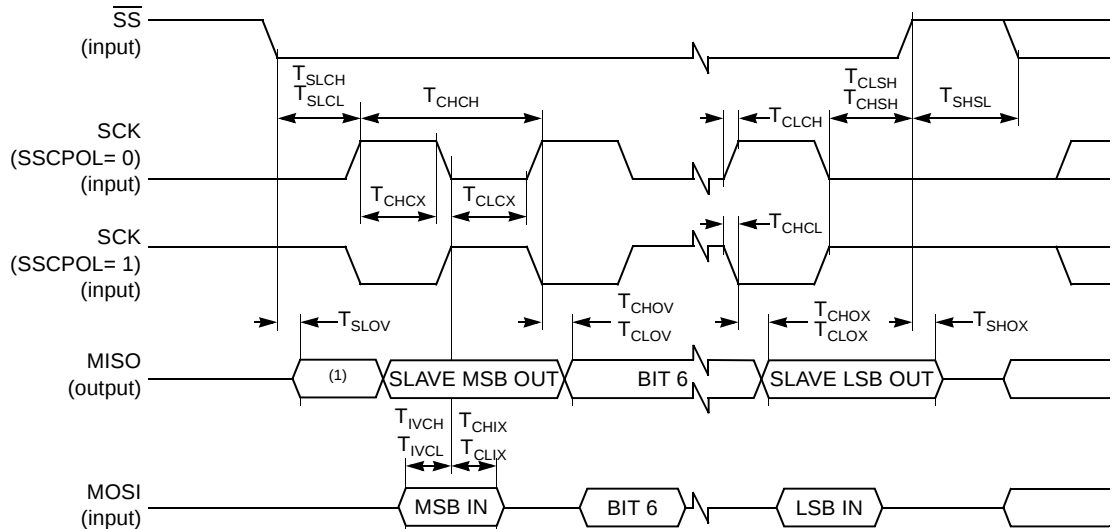
Figure 159. SPI Slave Waveforms (SSCPHA= 1)
